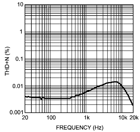
THD+N vs Frequency V_{DD} = 3V, R_L = 32\Omega, \text{One channel}, P_O = 50mW
