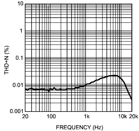
THD+N vs Frequency V_{DD} = 3V, R_L = 32\Omega, \text{Stereo}, P_O = 25mW
