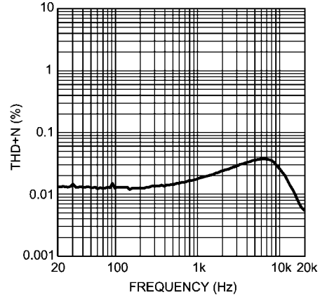
THD+N vs Frequency V_{DD} = 1.6V, R_L = 32\Omega, \text{Stereo}, P_O = 3mW
