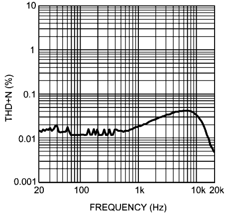
THD+N vs Frequency V_{DD} = 3V, R_L = 16\Omega, \text{Stereo}, P_O = 25mW
