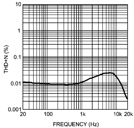
THD+N vs Frequency V_{DD} = 3V, R_L = 16\Omega, \text{One channel}, P_O = 60mW
