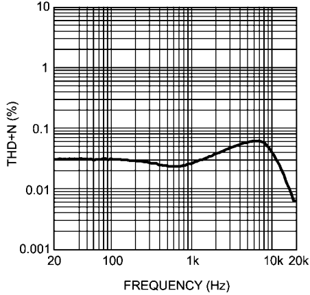
THD+N vs Frequency V_{DD} = 1.6V, R_L = 16\Omega, \text{Stereo}, P_O = 3mW
